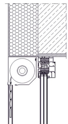
c installation in a recess with inverted box (curtain rolled inwards)
